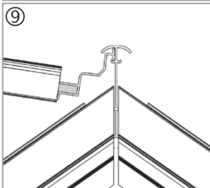
ADDITIONAL ROOF VENT V C
